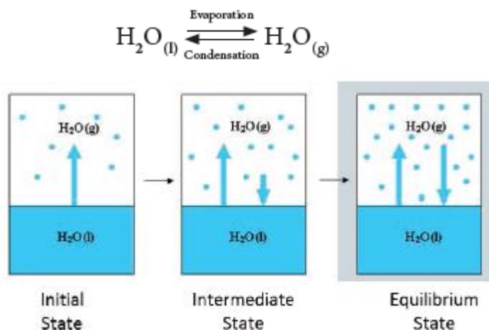
State of physical equilibrium
