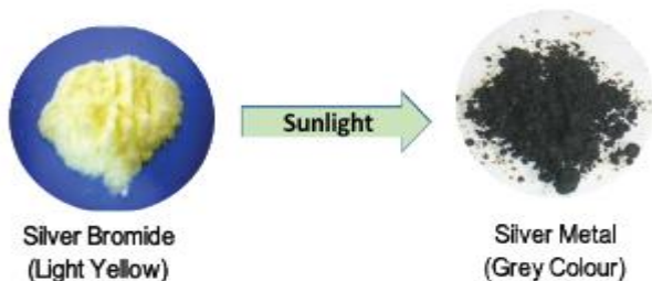
Photo decomposition of silver bromide
