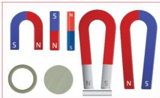
Artificial magnets
