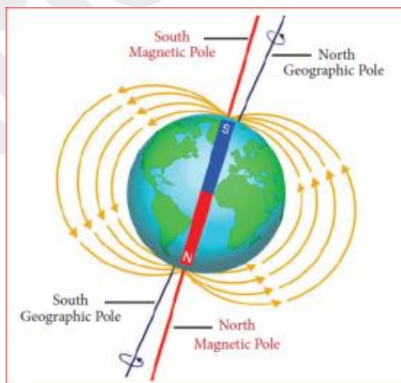
Earth as a magnet
