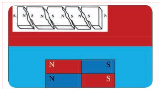
Magnetic poles exist in pair
