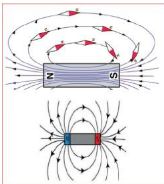
Magnetic Field
