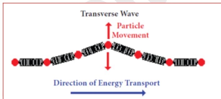
Transverse wave
