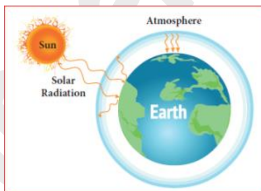
Greenhouse effect
