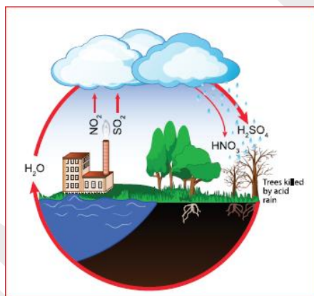
Acid Rain
